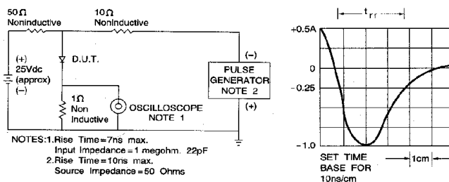
FIG. 5 - REVERSE RECOVERY TIME CHARACTERISTIC AND TEST DIAGRAM
