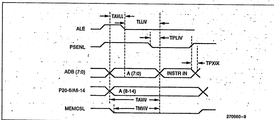
Figure 20. External Program Memory Read
