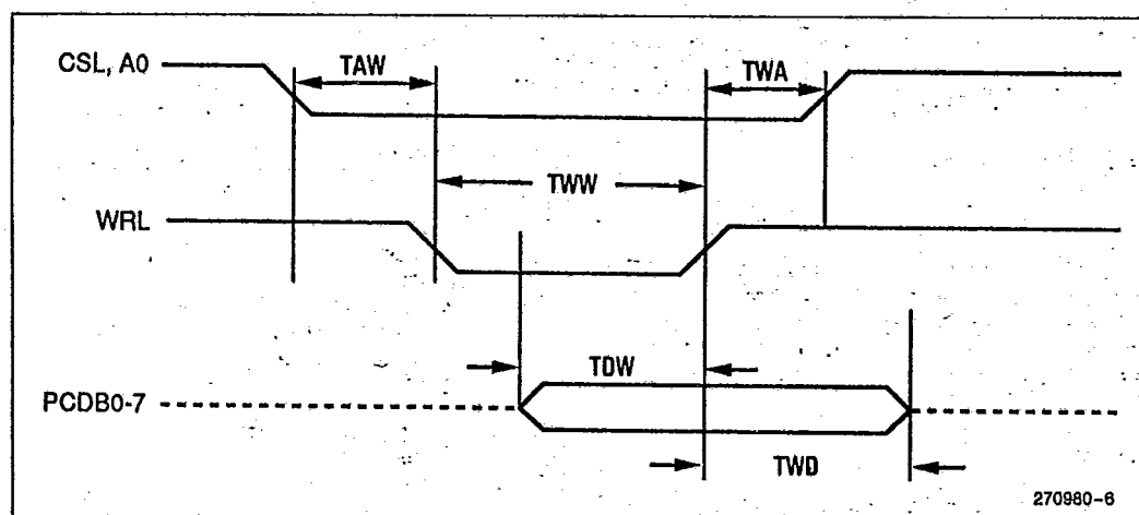
Figure 17. Host-Interface Write
