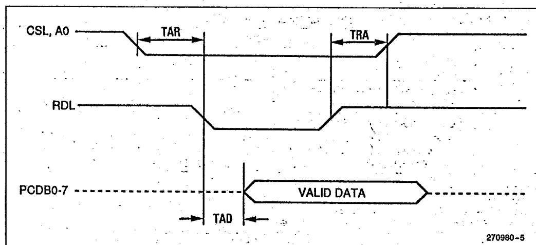
Figure 16. Host-Interface Read
