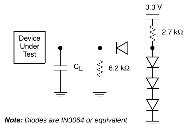
Figure 11. Test Setup
