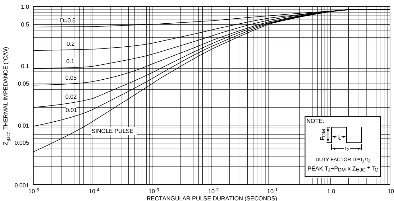
FIGURE 1, MAXIMUM EFFECTIVE TRANSIENT THERMAL IMPEDANCE, JUNCTION-TO-CASE vs PULSE DURATION
