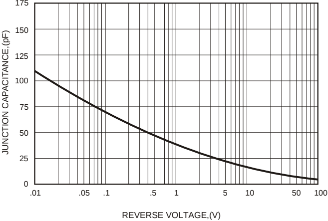
FIG.6-TYPICAL JUNCTION CAPACITANCE
