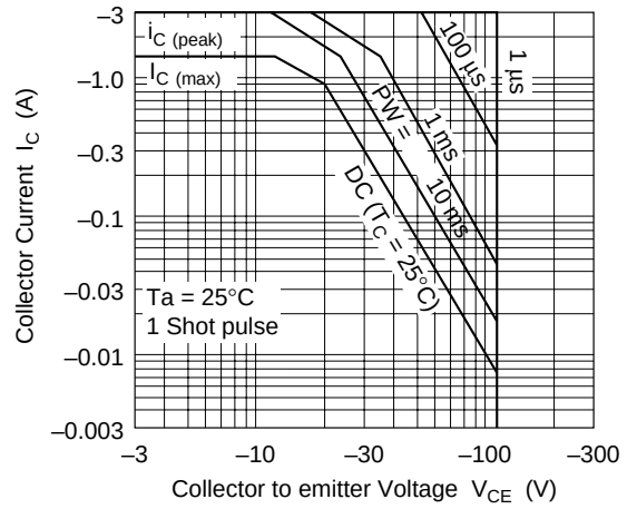
Area of Safe Operation
