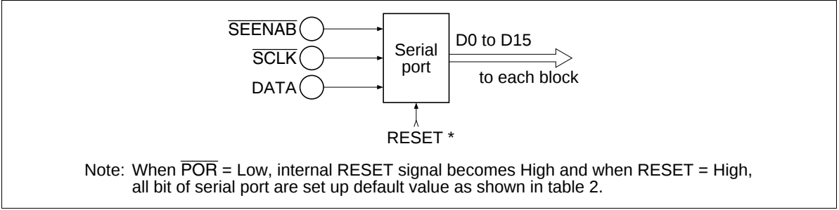
Figure 1 Construction of Serial Port
