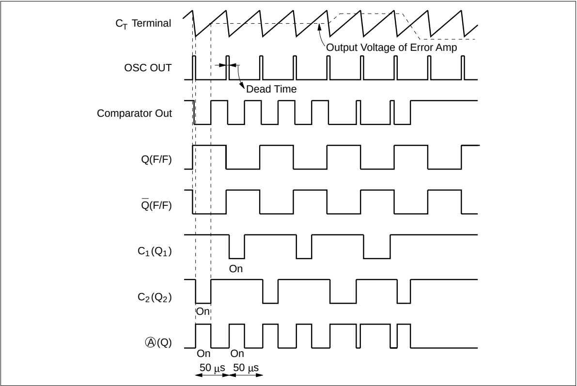
Figure 9 Operating Waveforms
