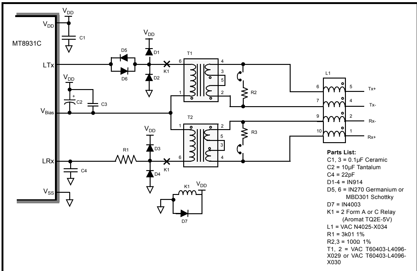
Figure 22 - ETS 300-012 NT &amp; TE Line Interface for VAC X029 or X030
