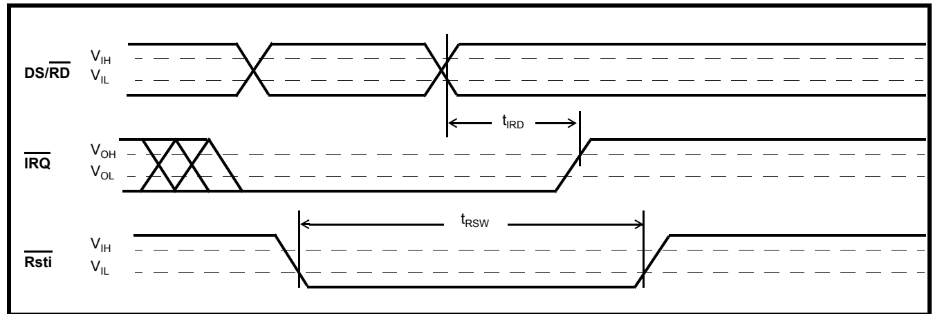
Figure 27 - INT &amp; Rsti Timing
