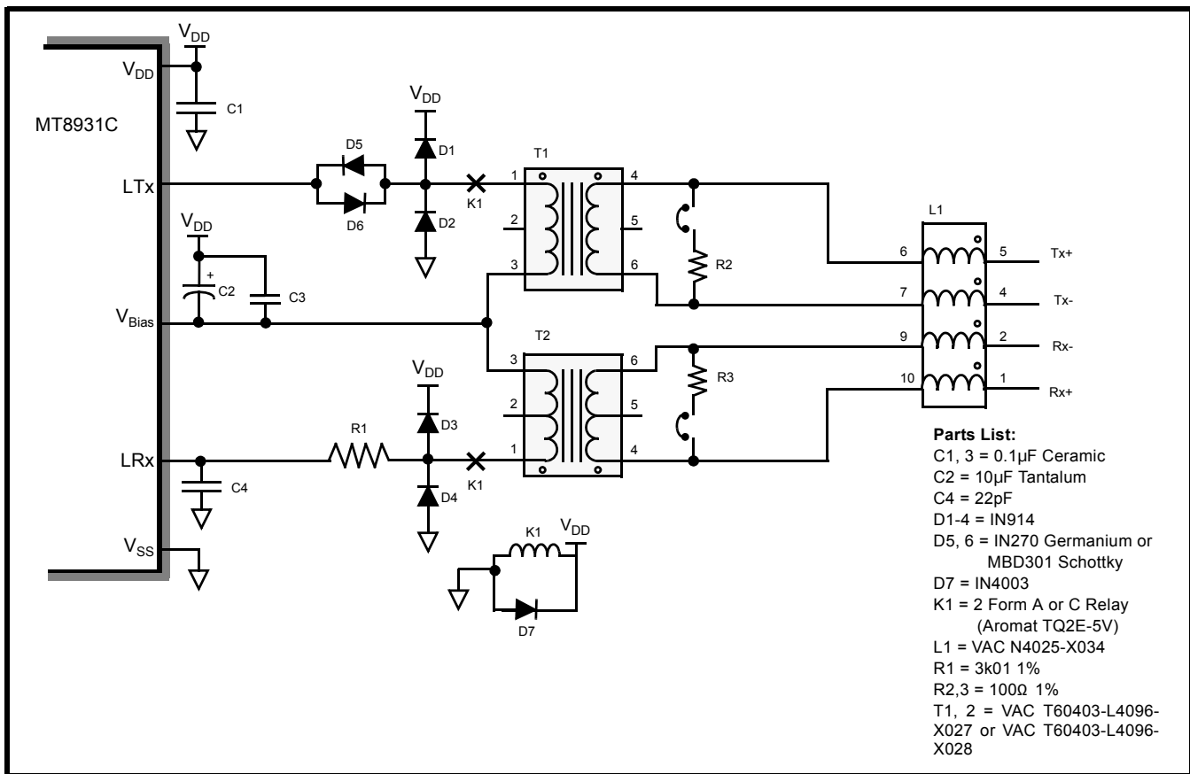
Figure 21 - ETS 300-012 NT &amp; TE Line Interface for VAC X027 or X028
