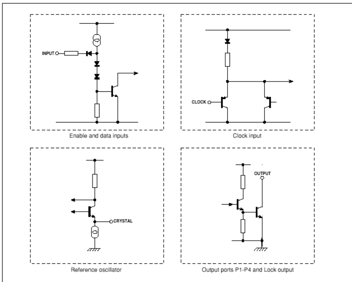
Figure 7 - Input/Output Interface Circuits
