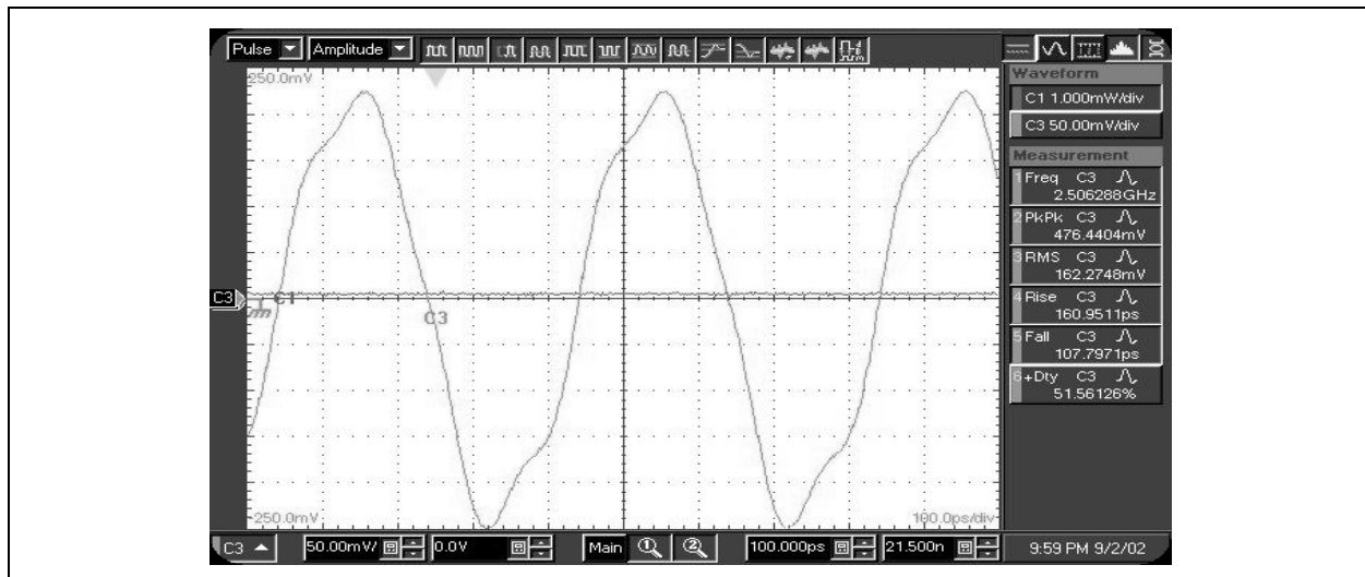
Figure 16 - Single-ended output waveform, showing some feedthrough of the input waveform.
