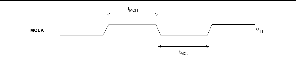
Figure 14 - Master Clock
