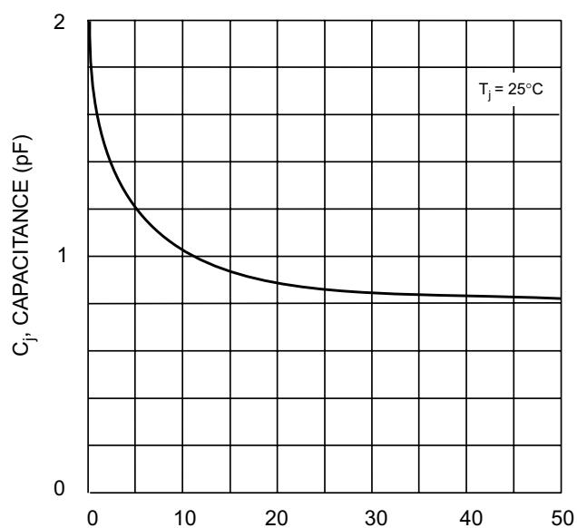
V_R , REVERSE VOLTAGE (V) Fig. 2 Typ. Junction Capacitance vs Reverse Voltage
