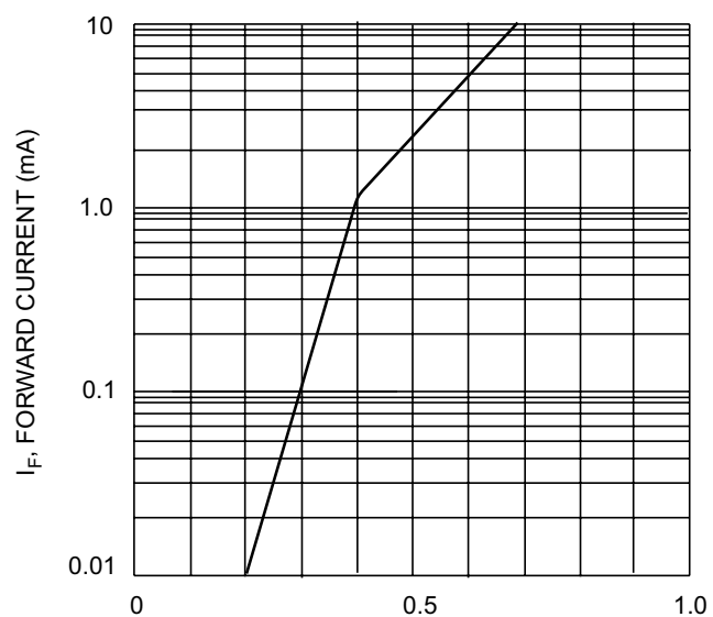
V_F , FORWARD VOLTAGE (V) Fig. 1 Typical Forward Characteristic Variations for Primary Conduction
