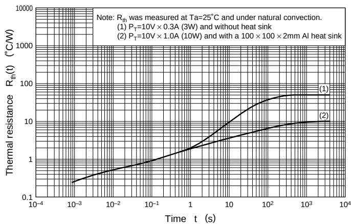
R_{th}(t) \text{ — } t
