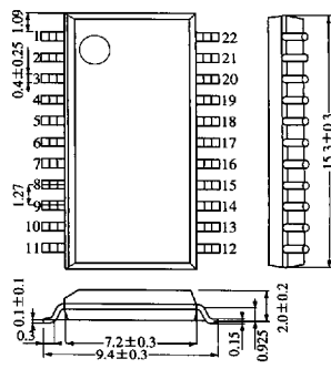
22-Pin PANAFLAT Package (SOP022-P-0375)
