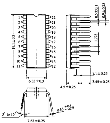
22-Pin Shrink DIL Plastic Package (SDIP022-P-0300A)
