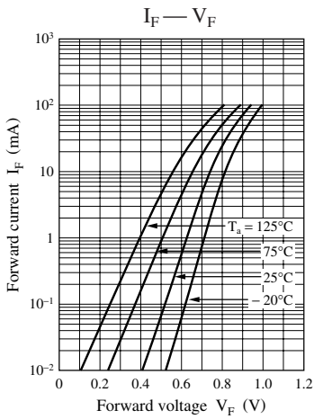
Characteristics chart of MA3X152A
