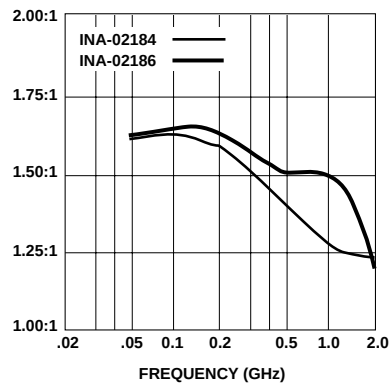
Figure 8. Output VSWR vs. Frequency, I_d = 35\text{ mA} .
