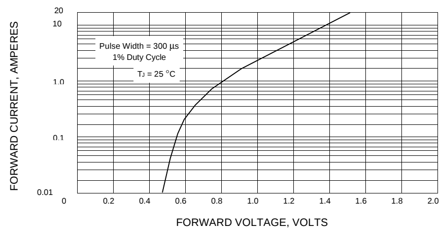
FIG.4 - TYPICAL FORWARD CHARACTERISTICS
