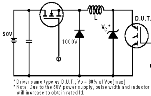
Fig. 13a - Clamped Inductive Load Test Circuit
