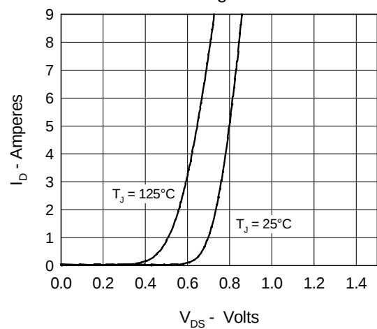
Fig.10 Source Current vs. Source to Drain Voltage
