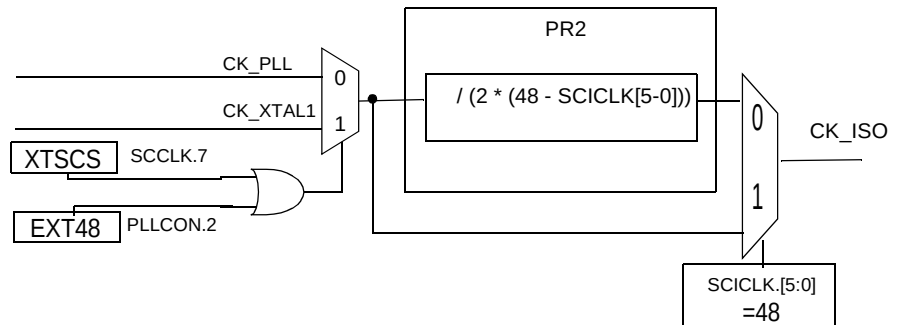
Figure 27. Prescaler 2 Description
