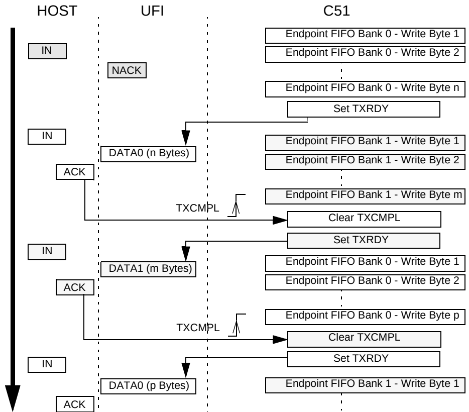
Figure 39. Bulk / Interrupt IN transactions in Ping-Pong mode
