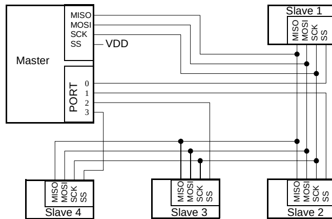
Figure 64. Typical SPI Bus
