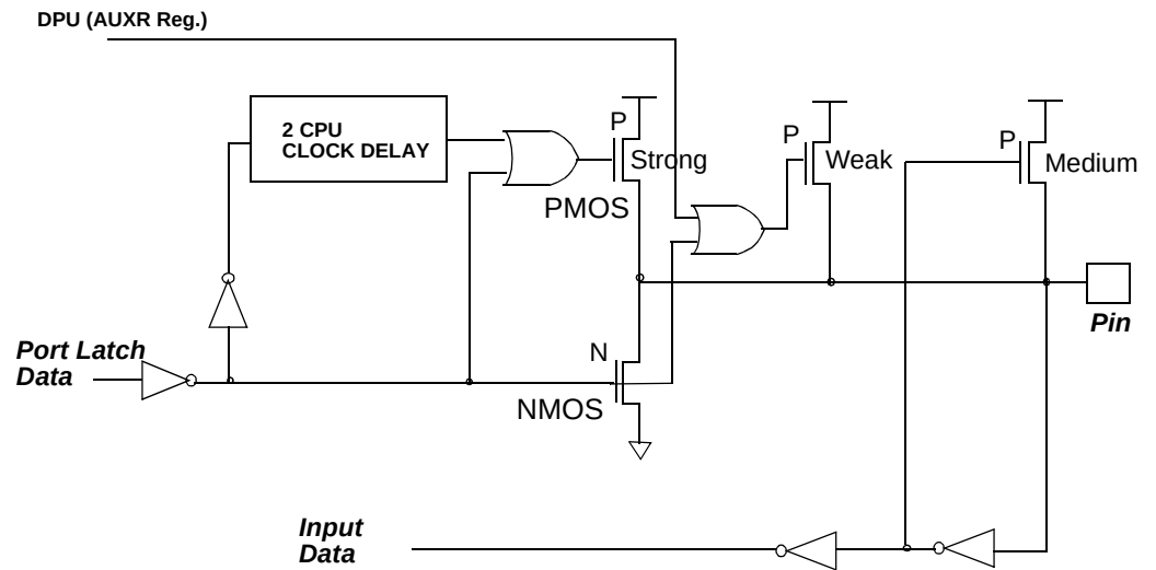
Figure 6. Quasi-Bi-directional Output
