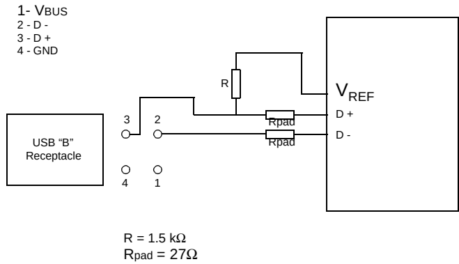
Figure 97. USB Interface
