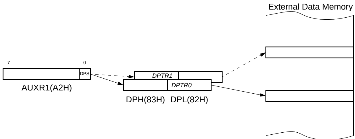
Figure 89. Use of Dual Pointer
