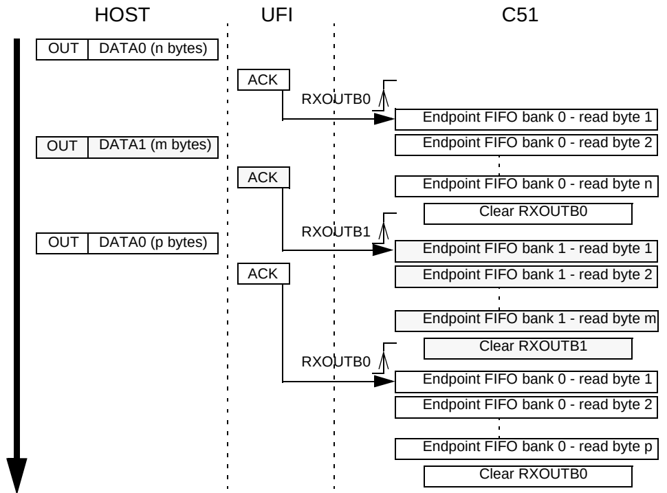
Figure 37. Bulk / Interrupt OUT transactions in Ping-Pong mode
