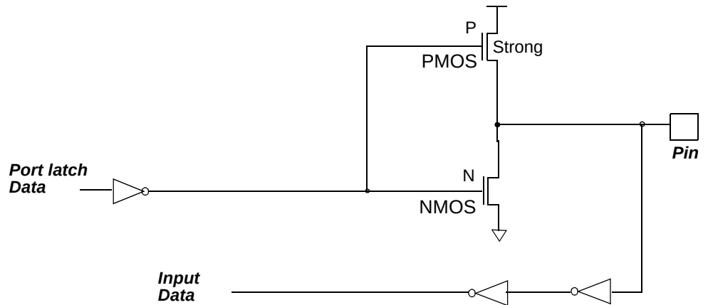
Figure 7. Push-pull Output
