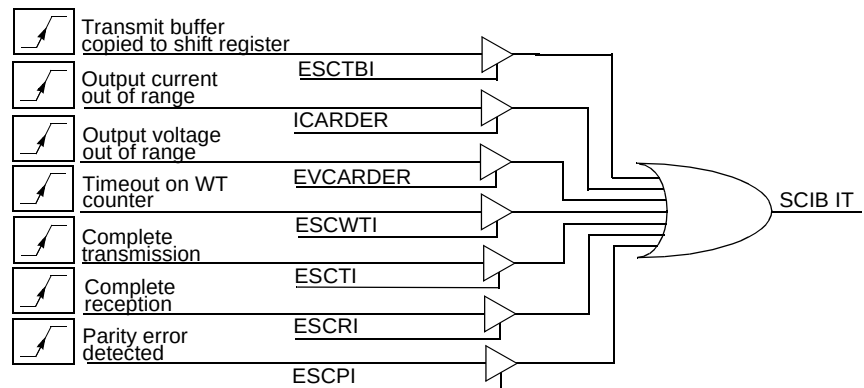
Figure 25. SCIB Interrupt Sources
