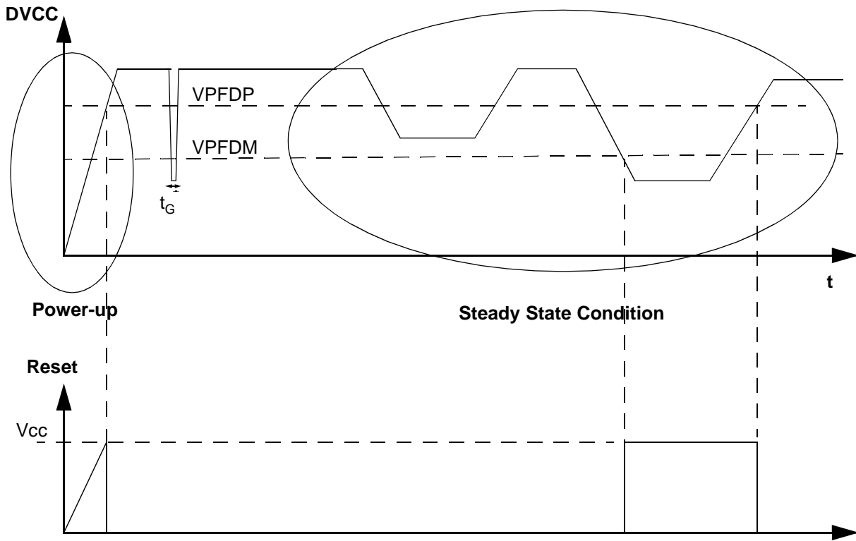
Figure 84. Power-up and Steady-state Conditions Monitored
