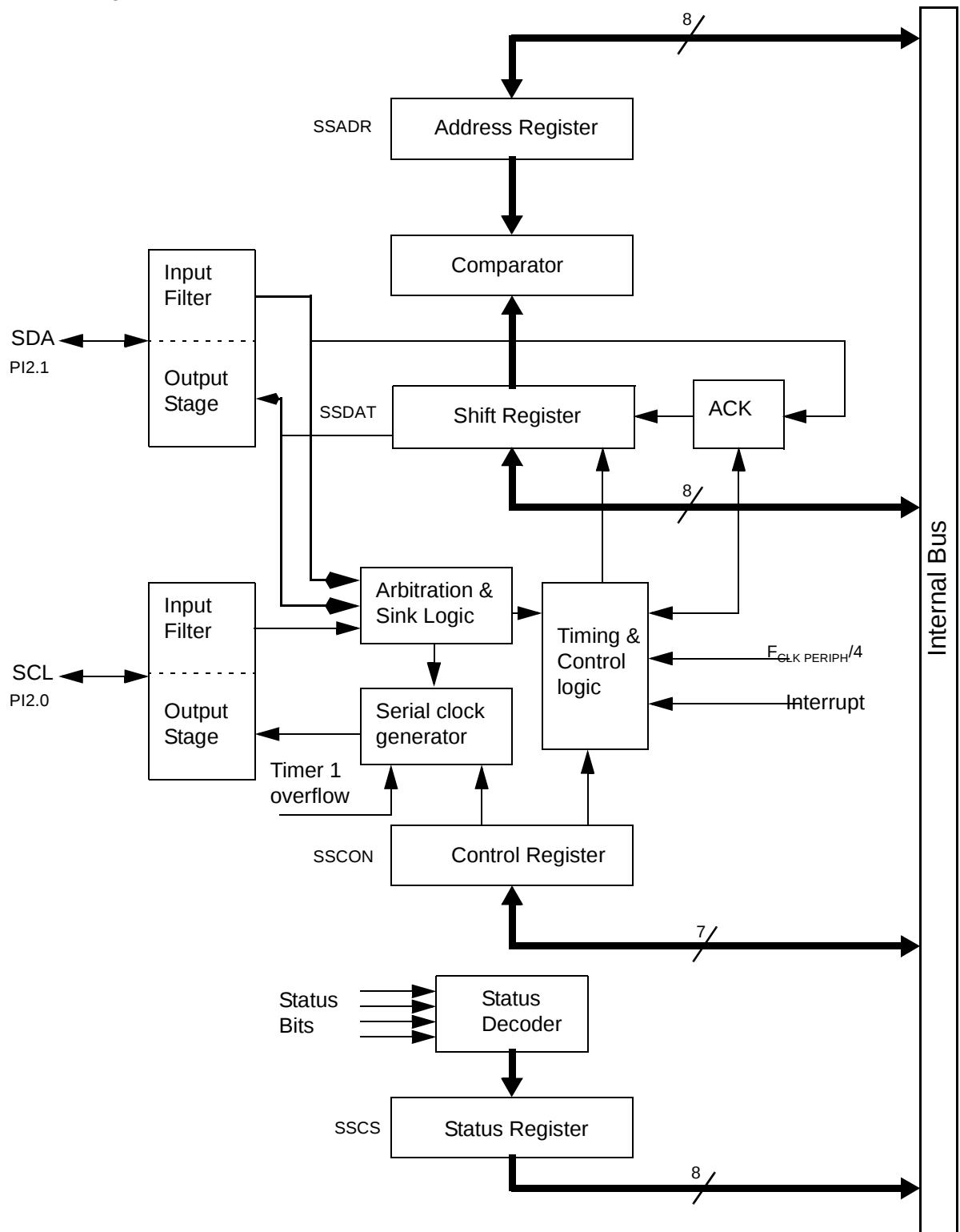
Figure 47. Block Diagram
