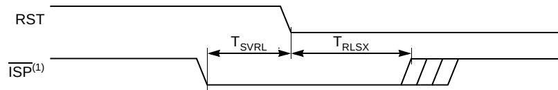
Figure 14. Flash Memory – ISP Waveforms
