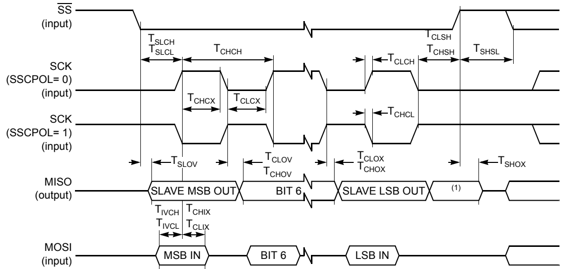
Figure 84. SPI Slave Waveforms (SSCPHA= 0)
