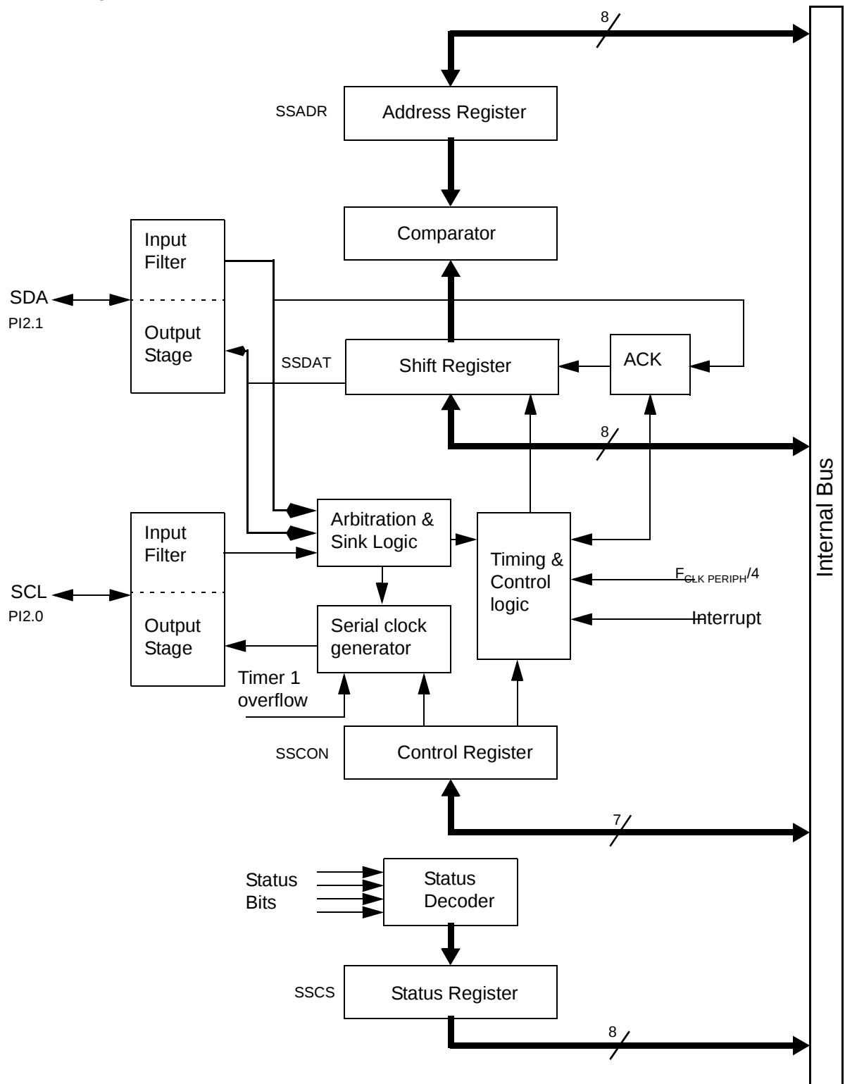
Figure 36. Block Diagram
