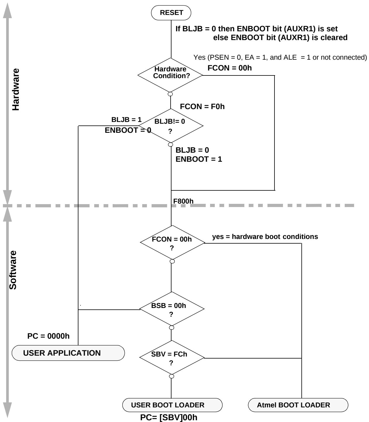
Figure 46. Bootloader process
