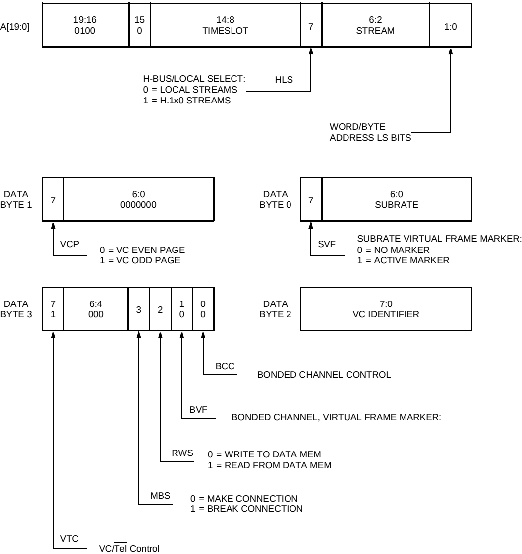
Figure 44. Microprocessor Programming—Make/Break/Query Virtual Channel Nonbonded Connections
