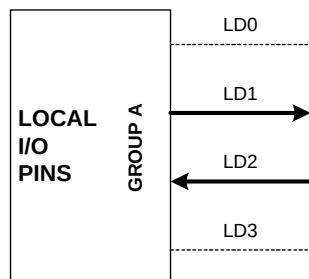
GROUP A CONFIGURATION 3 AT 16.384 Mbits/s SUPERRATE
