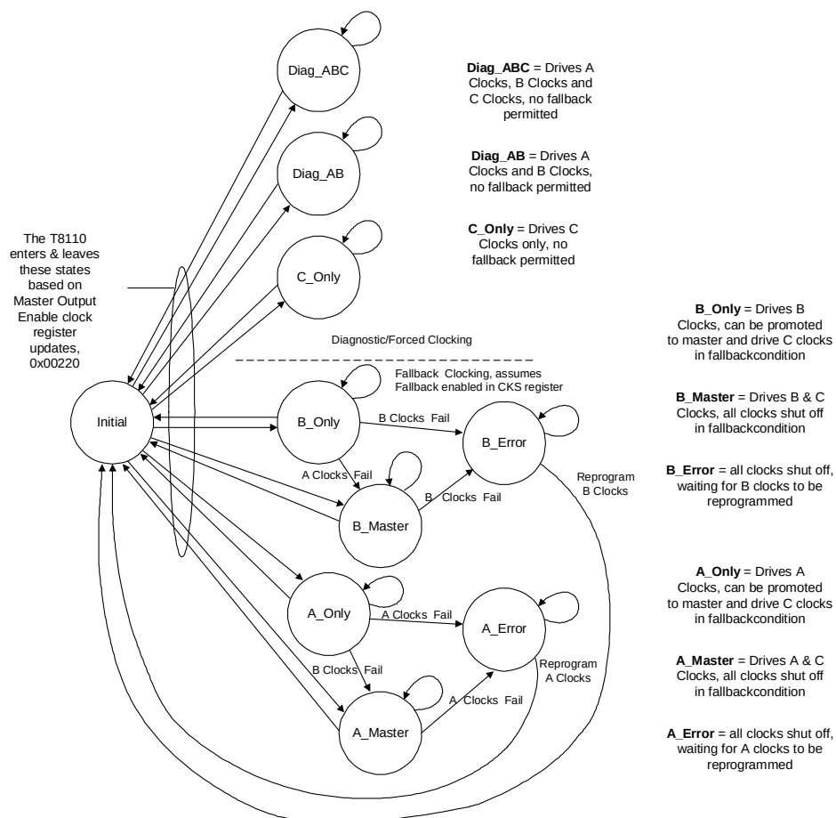
Figure 24. T8110 H-Bus Clock Enable States
