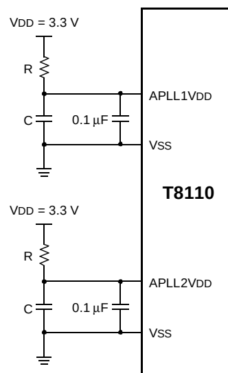
Figure 62. APLL VDD Filtering
