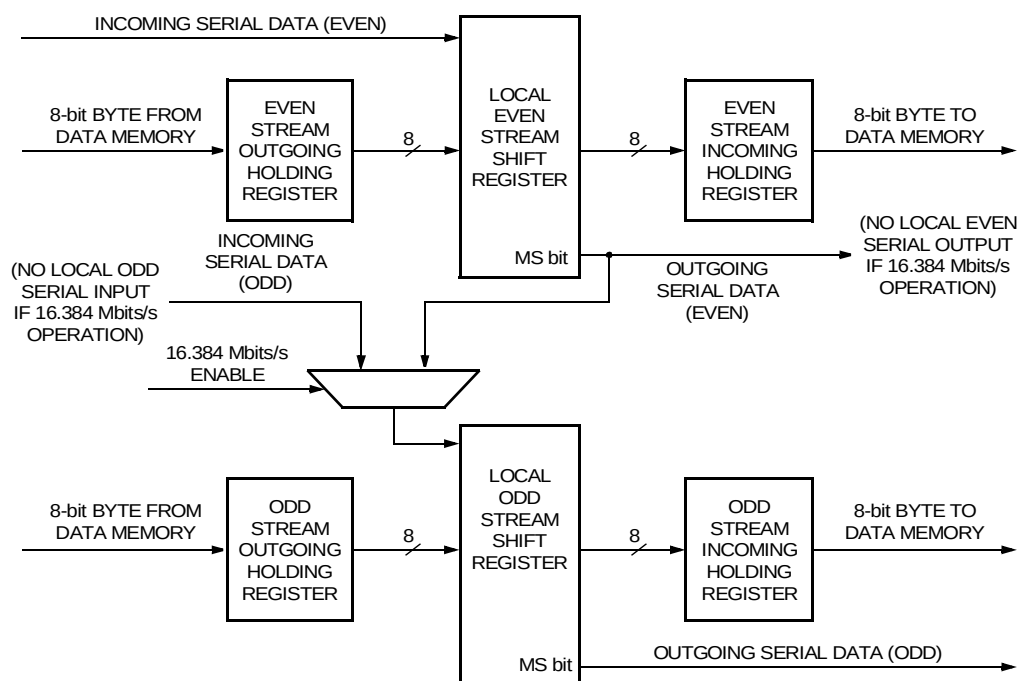
Figure 30. Local Stream 16.384 Mbits/s Circuit
