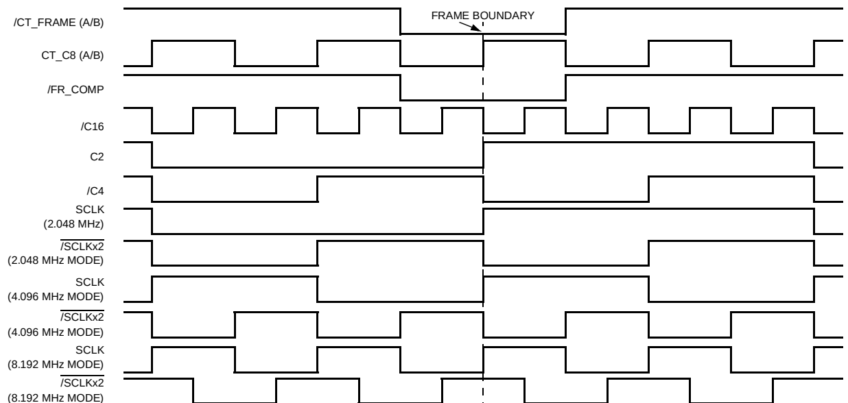
Figure 59. Clock Alignment
