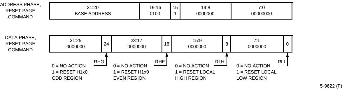
Figure 35. PCI Programming—Reset Page Command
