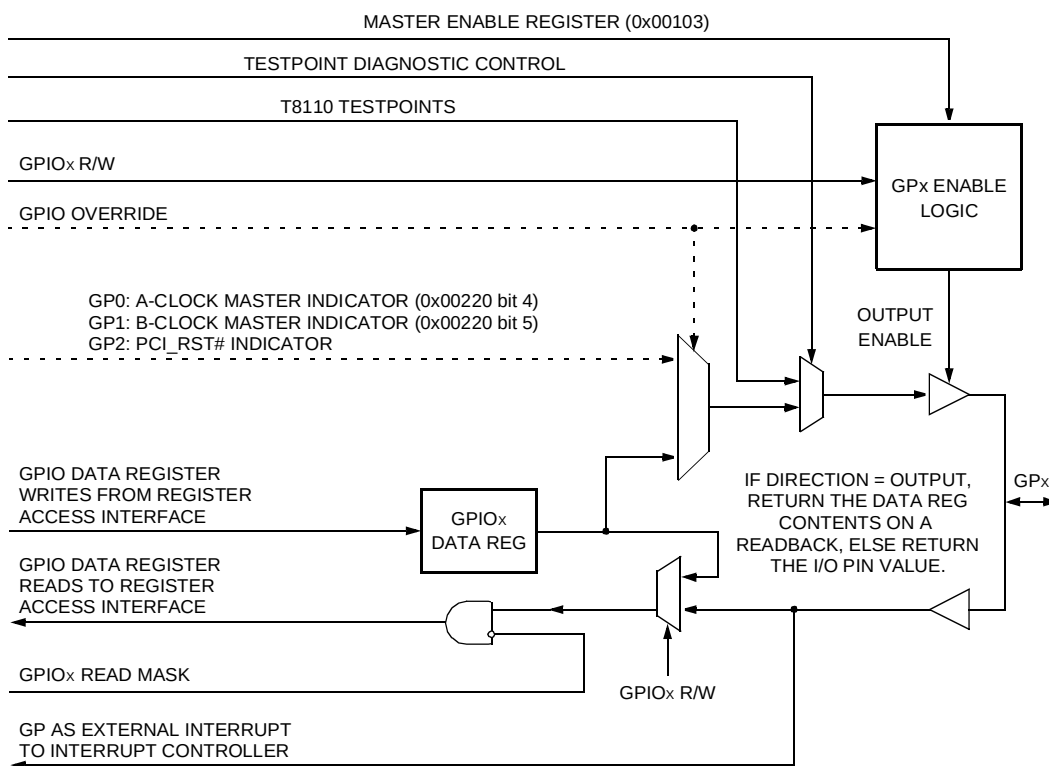
Figure 28. GP[7:0] Functional Paths
