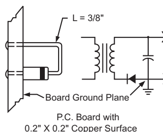
MOUNTING METHOD
