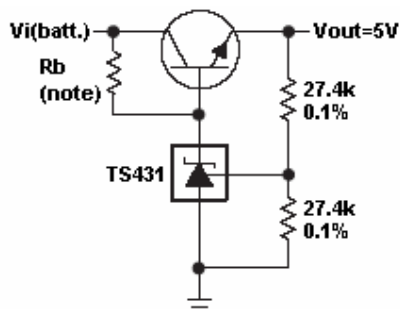
Figure 14. Efficient 5V Precision Regulator
