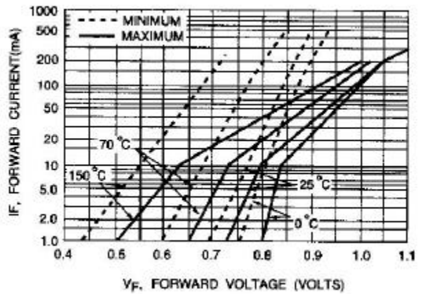
Fig. 10-TYPICAL FORWARD CHARACTERISTICS
