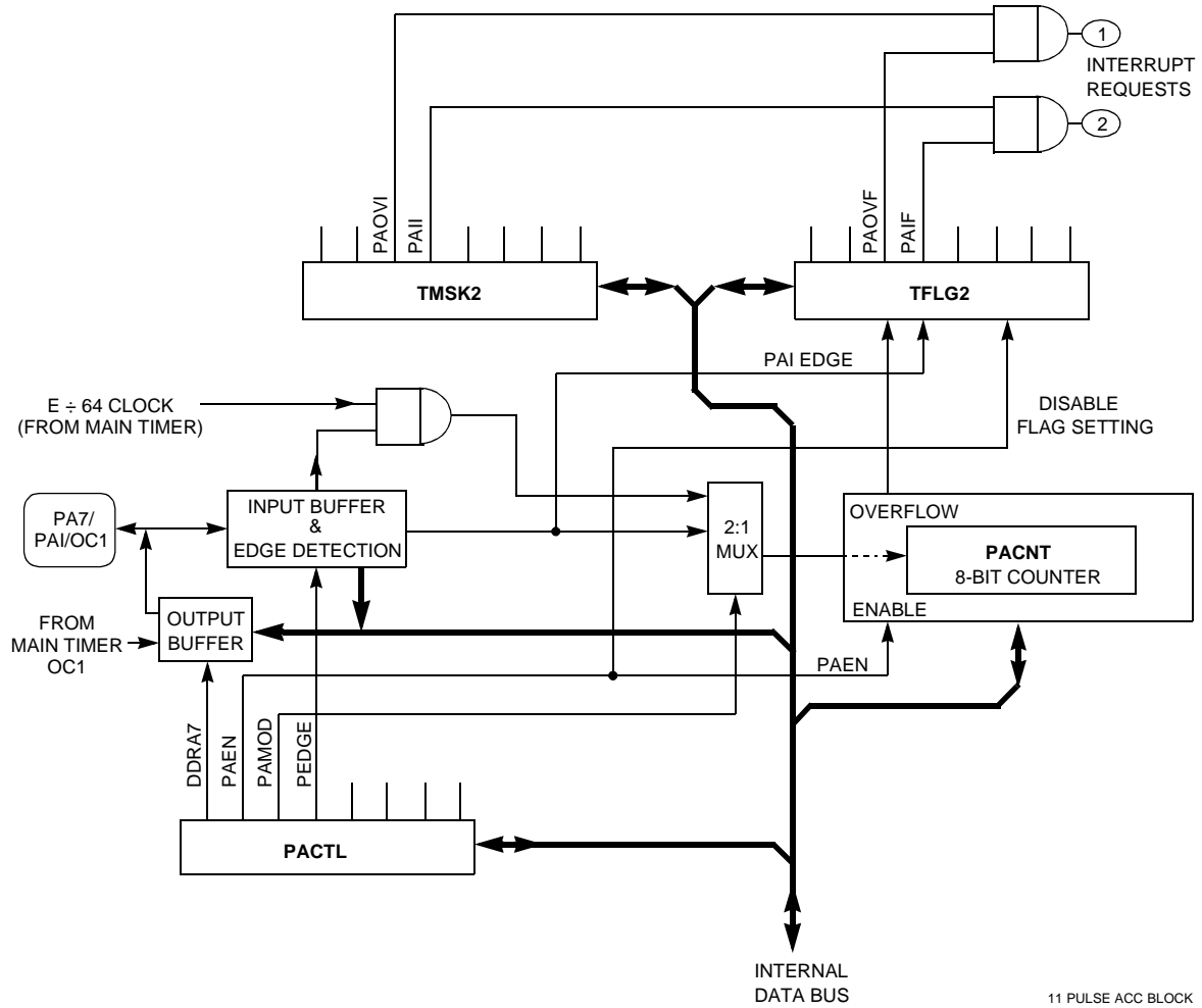
Figure 9-3 Pulse Accumulator
