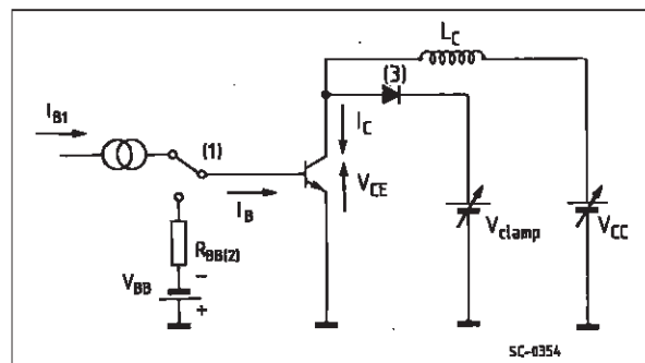
RBSOA and Inductive Load Switching Test Circuit
