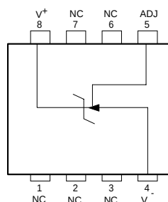
SO8 (Top view)
