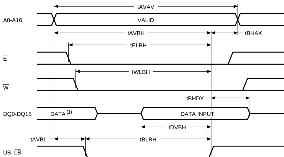
Figure 12. \overline{UB}/\overline{LB} Controlled, Write AC Waveforms
