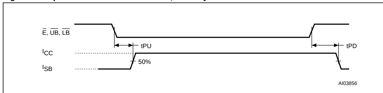
Figure 9. Chip Enable or \overline{UB}/\overline{LB} Controlled, Standby Mode AC Waveforms
