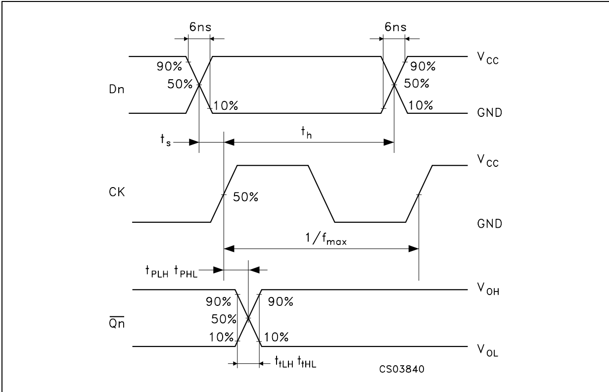
WAVEFORM 1: CK TO \overline{Qn} PROPAGATION DELAYS, Dn TO CK SETUP AND HOLD TIMES, CK MAXIMUM FREQUENCY (f=1MHz; 50% duty cycle)
