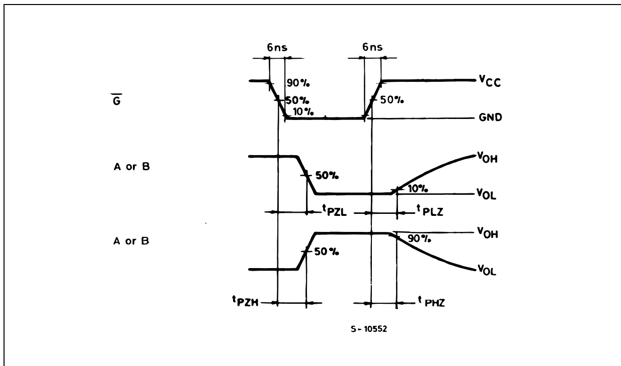
WAVEFORM 4 : OUTPUT ENABLE AND DISABLE TIME (f=1MHz; 50% duty cycle)
