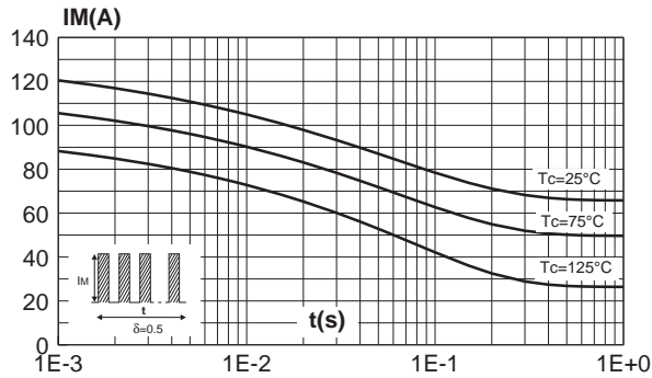
Fig. 3-1: Non repetitive surge peak forward current versus overload duration (maximum values, per diode, TO-220AB, TO-247, D 2 PAK).
