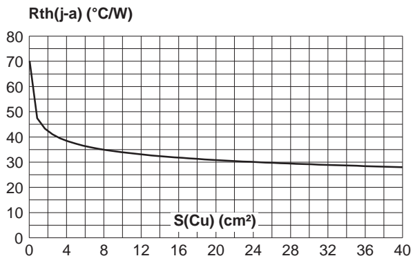
Fig. 8: Thermal resistance junction to ambient versus copper surface under tab (Epoxy printed circuit board FR4, copper thickness: 35\mu\text{m} ) ( D^2\text{PAK} ).
