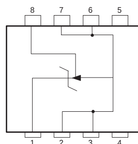
SO8 (Top view)
