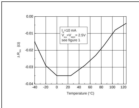
Drift of R_{KA} vs Temperature
