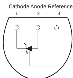
TO92 (Top view)
