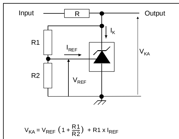
Figure 2 : Test Circuit for V_{KA} > V_{REF}
