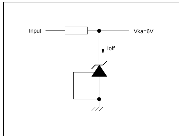
Test circuit for Vka &gt; Vref
