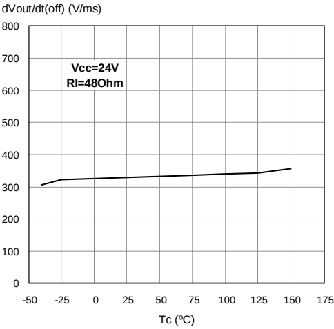
Figure 21. Turn-off Voltage Slope
