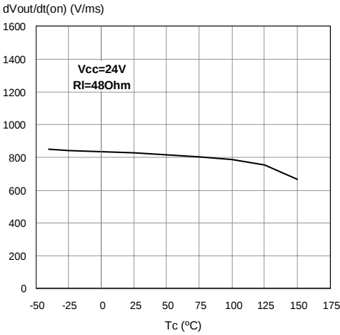
Figure 18. Turn-on Voltage Slope
