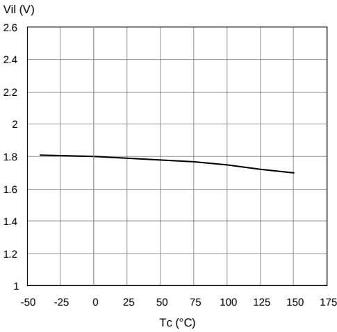
Figure 17. Input Low Level
