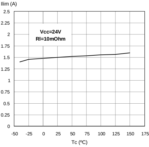
Figure 22. I LIM Vs T case
