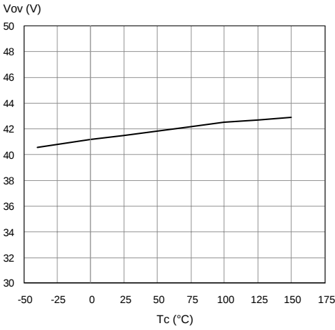
Figure 19. Overvoltage Shutdown
