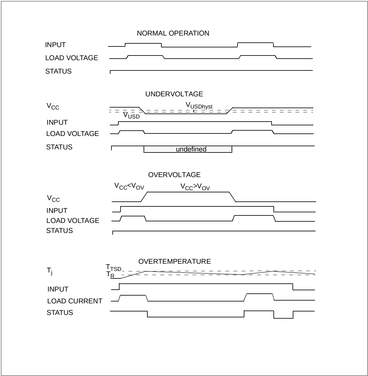
Figure 3: Waveforms
