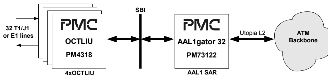
Figure 3 – High Density Leased Line Circuit Emulation Application
