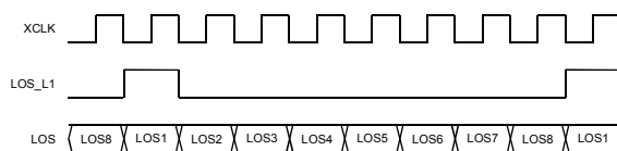
Figure 30 – LOS Alarm Serial Output
