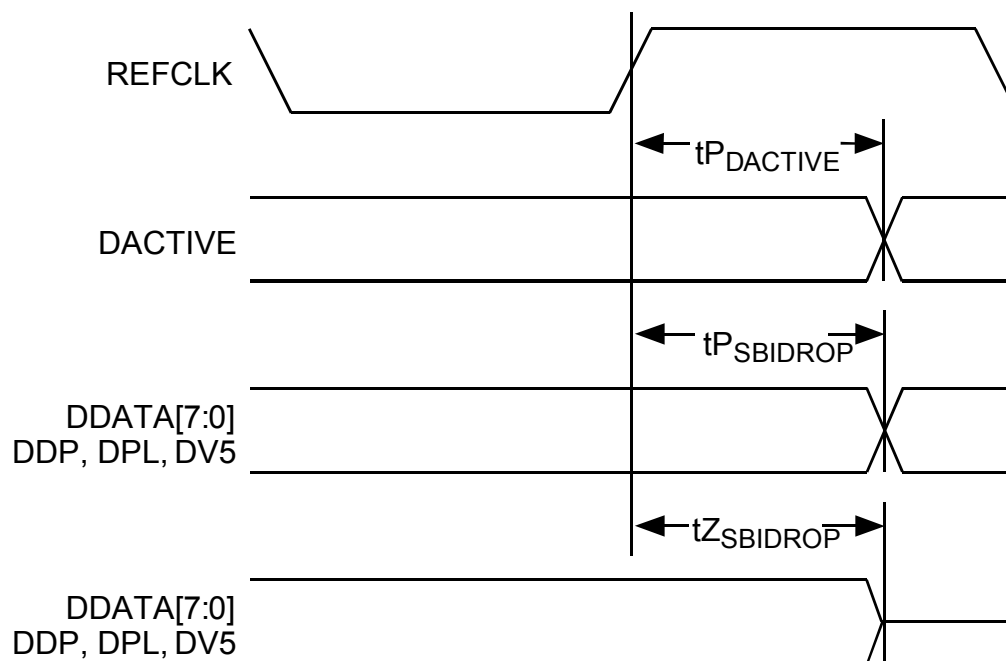
Figure 39 – SBI DROP BUS Timing
