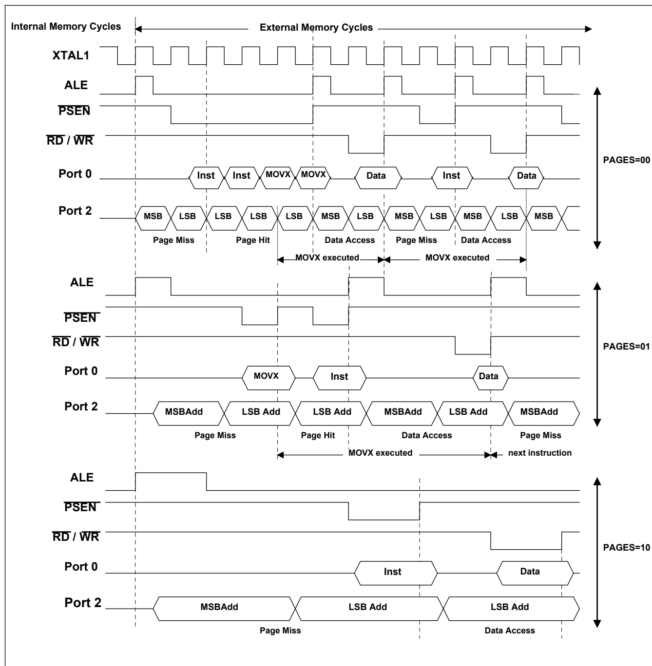
Figure 7. Page Mode 1, External Memory Cycle (CD1:CD0 = 10)
