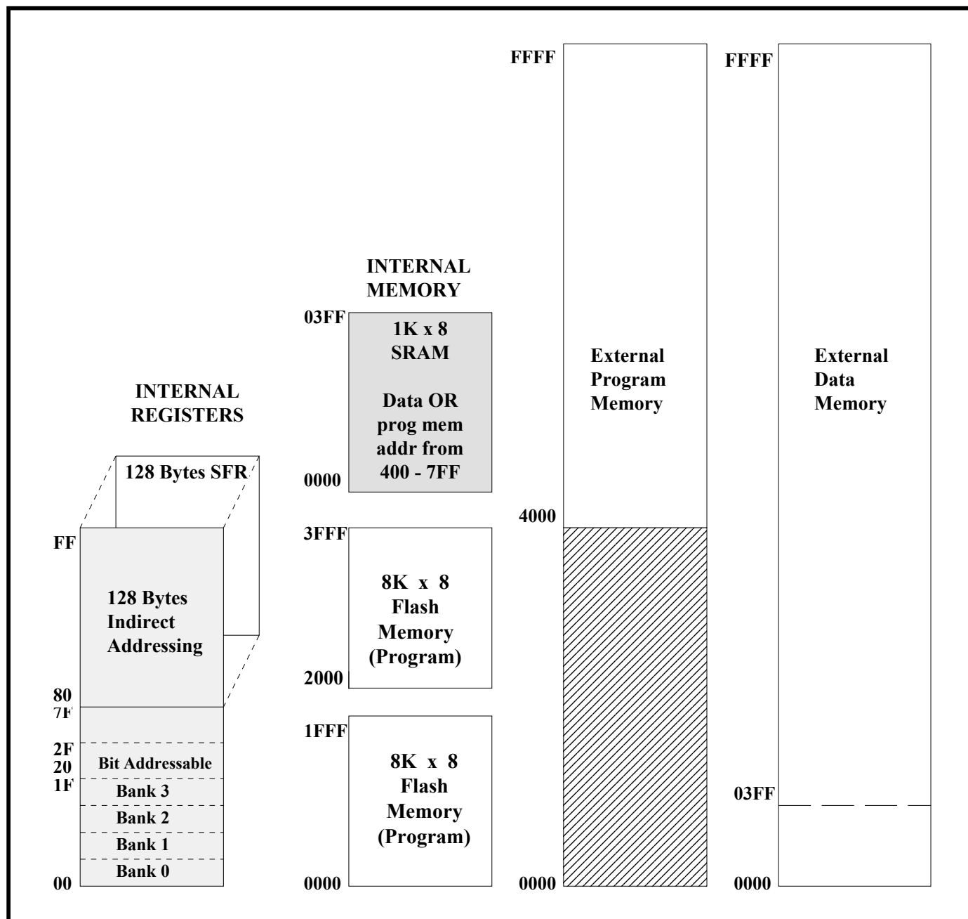
Figure 2. Memory Map
