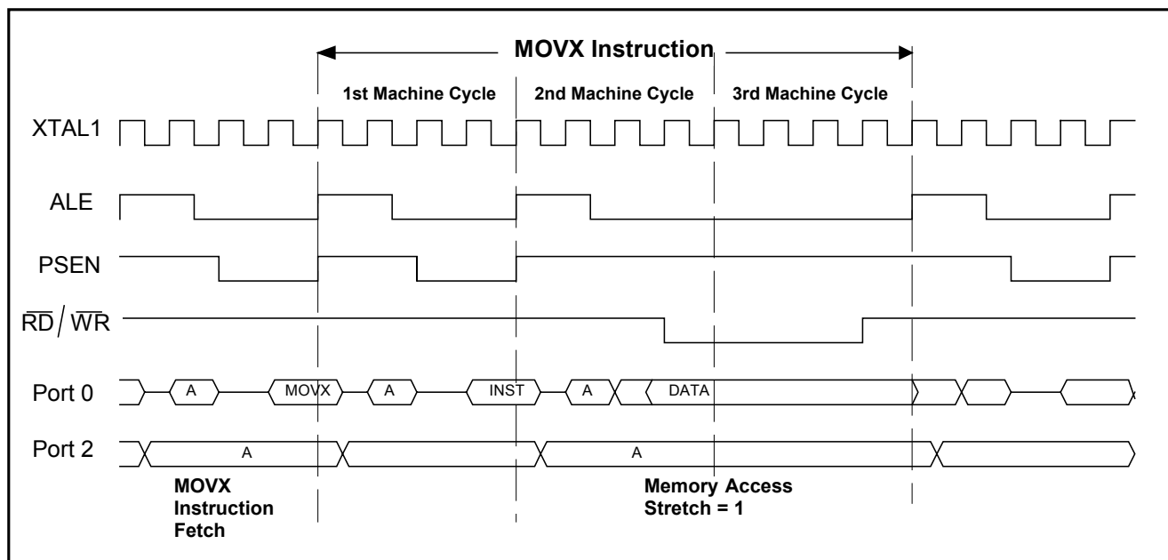
Figure 6. Non-Page Mode, External Data-Memory Access (Stretch = 1, CD1:CD2 = 10)
