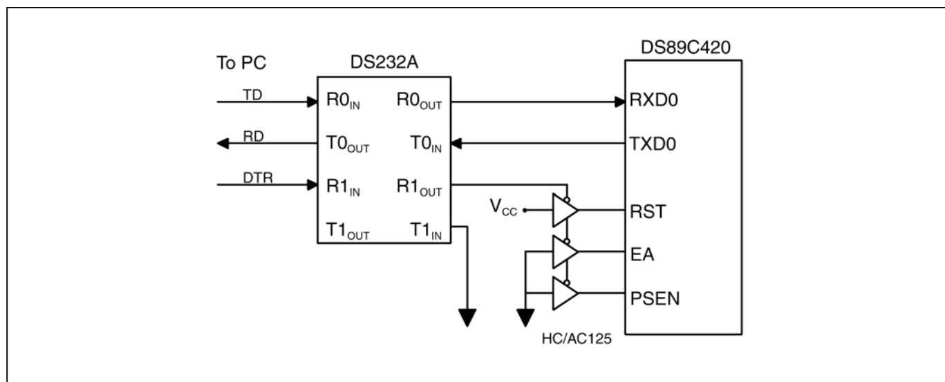
Figure 3. Interfacing the Bootloader to a PC
