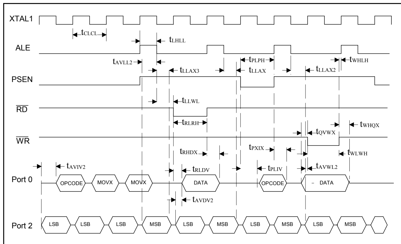
Figure 13. Page-Mode 1 Timing
