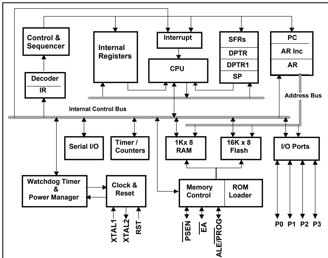
Figure 1. Block Diagram
