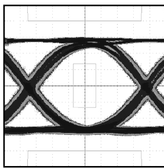
ELECTRICAL EYE DIAGRAM ( I_{MOD} = 100mA , 2^{13} - 1 + 80CID )
