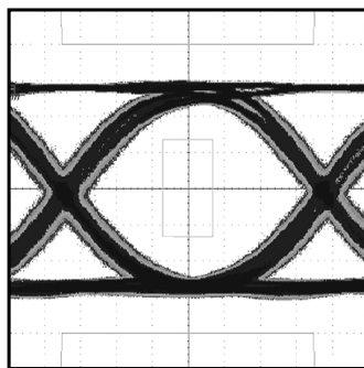
ELECTRICAL EYE DIAGRAM ( I_{MOD} = 100mA , 2^{13} - 1 + 80CID )
