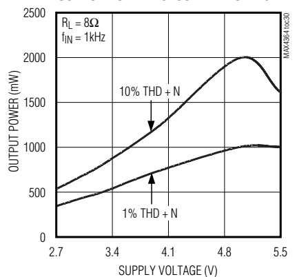
MAX4365 OUTPUT POWER vs. SUPPLY VOLTAGE
