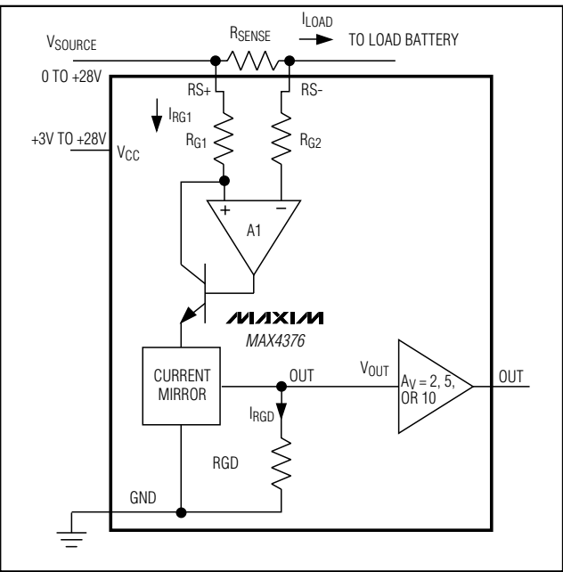
Figure 1. Functional Diagram
