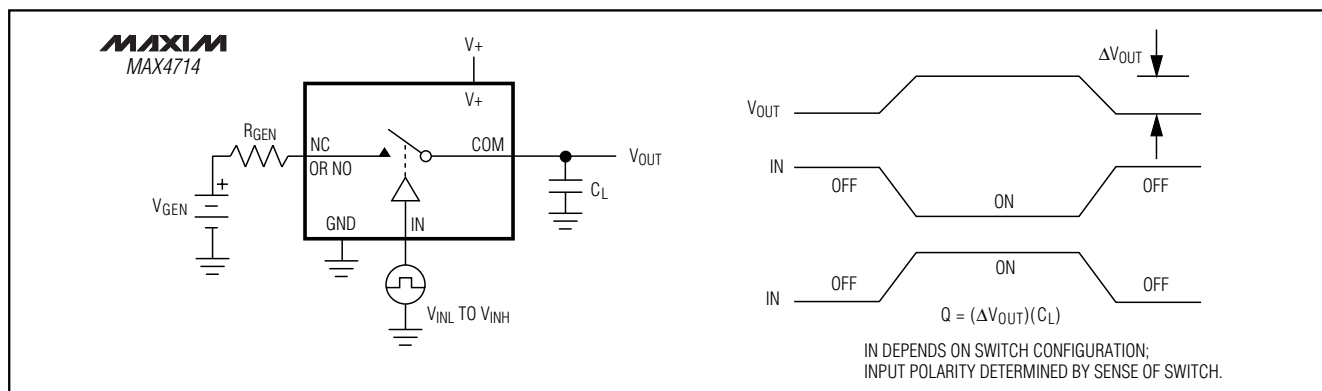
Figure 3. Charge Injection
