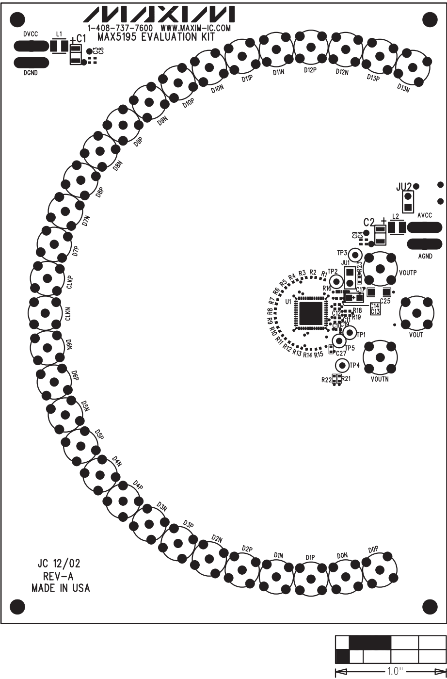
Figure 3. MAX5195 EV Kit Component Placement Guide—Component Side
