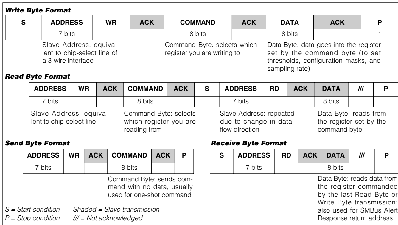
Figure 3. SMBus Protocols
